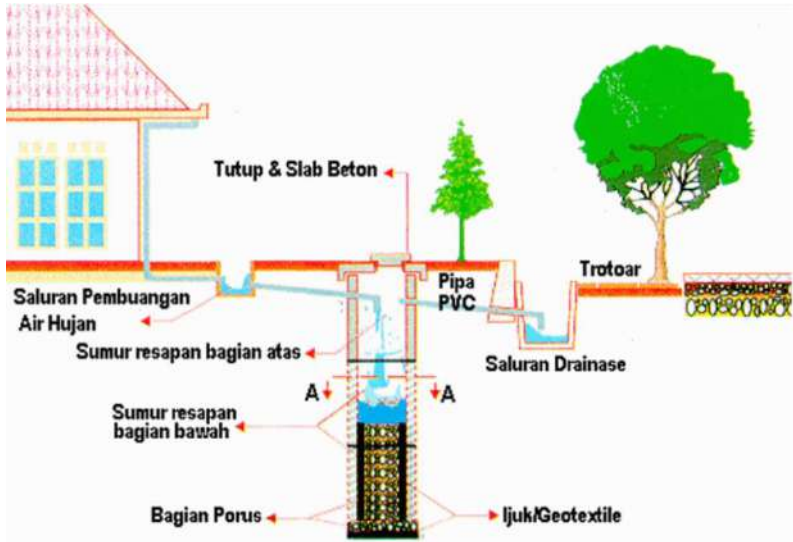
Gambar 5.13. Sumur Resapan ( Infiltration Well ) (Sumber : Kusdiawan, W, 2021)
