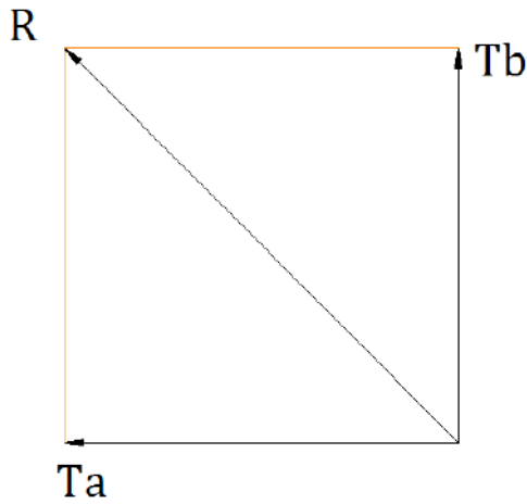
Gambar 5.5. Resultan Gaya
